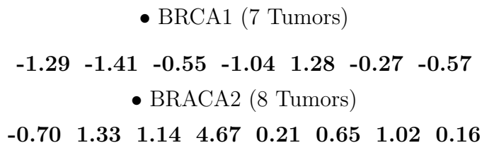
Figure 1: Expression data for the first of 3226 genes, microarray study of breast cancer; Hedenfalk et al. (2001).
